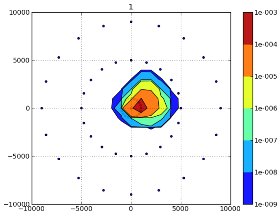
Figure: Asimilace v case t=20\text{min} .
