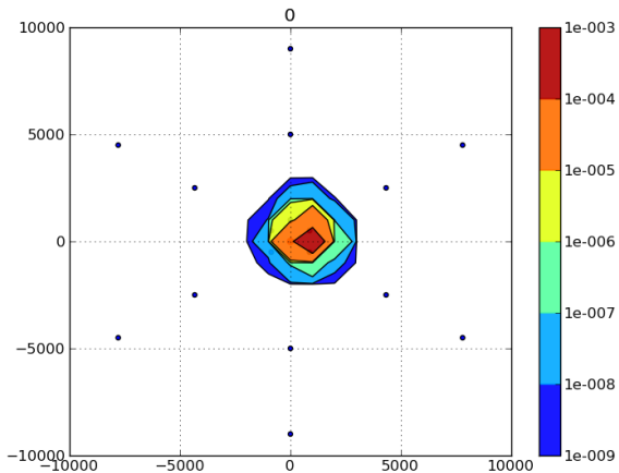
Figure: Asimilace v case t=10\text{min} .
