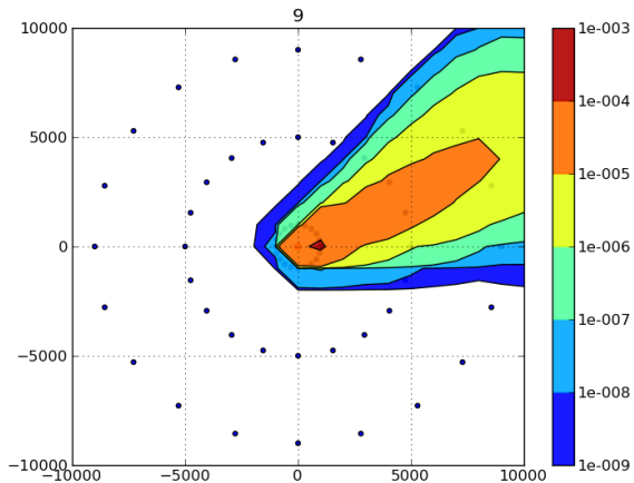
Figure: Asimilace v case t=100\text{min} .
