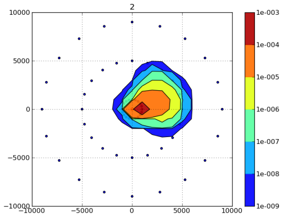
Figure: Asimilace v case t=30\text{min} .
