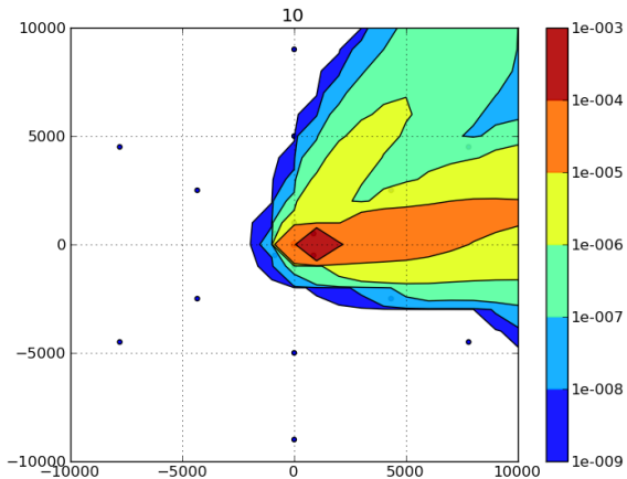
Figure: Asimilace v case t=110 min.
