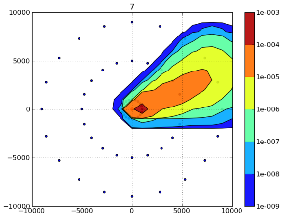
Figure: Asimilace v case t=80\text{min} .
