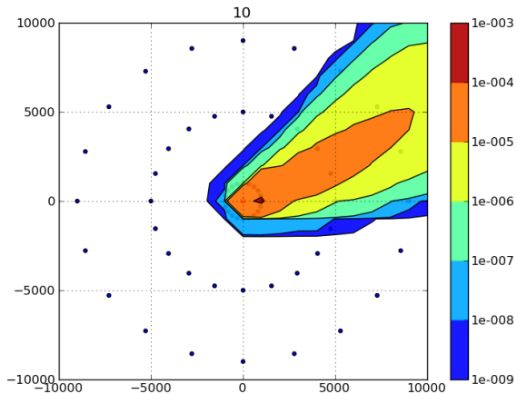
Figure: Asimilace v case t=110\text{min} .
