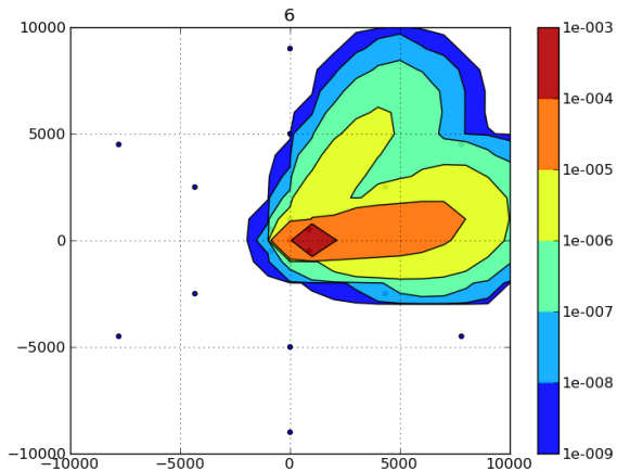
Figure: Asimilace v case t=70 min.
