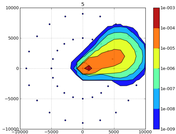
Figure: Asimilace v case t=60\text{min} .
