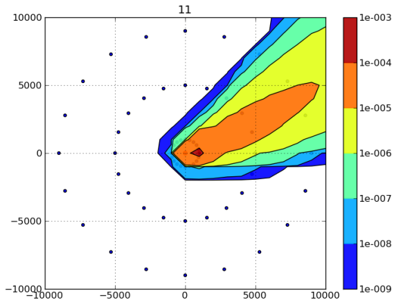
Figure: Asimilace v case t=120 min.
