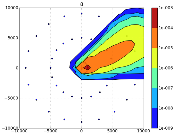
Figure: Asimilace v case t=90\text{min} .
