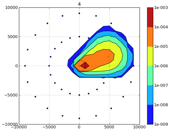
Figure: Asimilace v case t=50 min.
