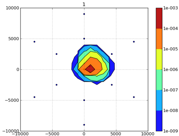
Figure: Asimilace v case t=20 min.
