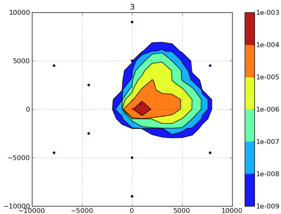
Figure: Asimilace v case t=40 min.
