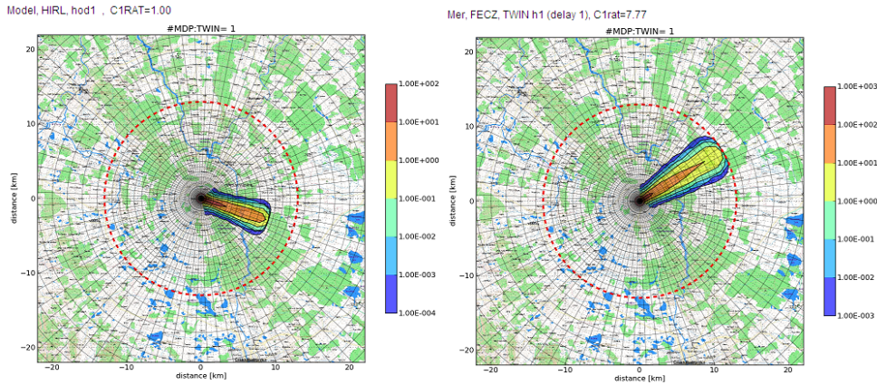
Figure 4.7: Assimilation in the first hour: "Best estimate" (left) and TWIN (right) trajectories. TWIN: c_1=7.77 c_\varphi=-46.90 c_{u10}=1.00 ; Assimilated values reached after 124 iterations: IFCN=124, c_1=7.768 c_\varphi=-47.96 c_{u10}=0.999 .
