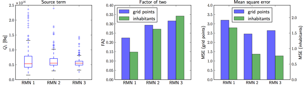
Figure 4.6: Results of network assessment. Left: Boxplots of estimated magnitudes of release given by the ensemble for all three monitoring networks. We observe that median for all networks is sufficiently close to the true value 5.0E+15 Bq of ^{137}\text{Cs} . Middle-Right: Values of loss functions. RMN 2 with regularly spaced receptors attained higher value of FA2 (grid points) over FA2 (inhabitants). RMN 3 with receptors placed in the inhabited sites attains higher value of FA2 (inhabitants).
