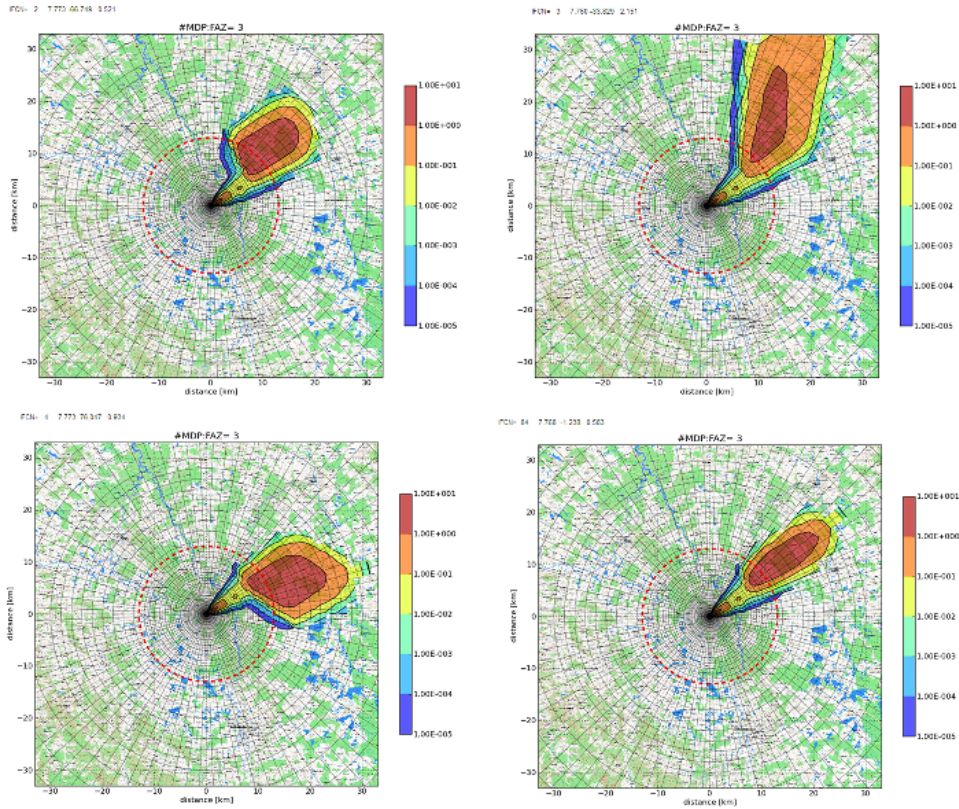
Figure 4.9: Assimilation in the third hour: Upper-left: The trajectory of dose rate in the beginning of the minimalisation procedure for IFCN=2 : c_1=7.773 , c_\varphi = -66.749 , c_{u10} = 0.521 . Upper-right: Trajectory IFCN=3 : c_1=7.760 , c_\varphi = -33.829 , c_{u10} = 2.151 . Lower-left: IFCN=4 : c_1=7.773 , c_\varphi = +76.047 , c_{u10} = 0.934 . Lower-right: The convergence is reached after the 84 iterations: IFCN=84: c_1=7.768 , c_\varphi = -1.238 , c_{u10} = 0.583 .
