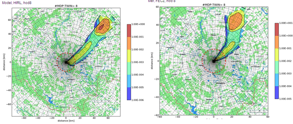
Figure 4.1: "Best estimate" (left) and TWIN (right) trajectories.
